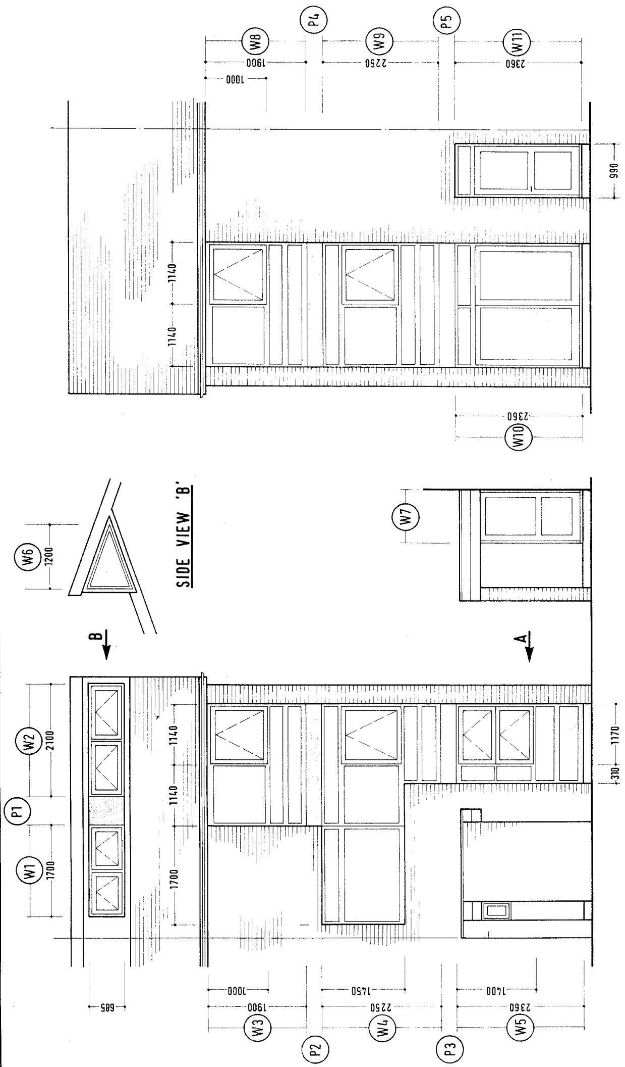
REAR ELEVATION
