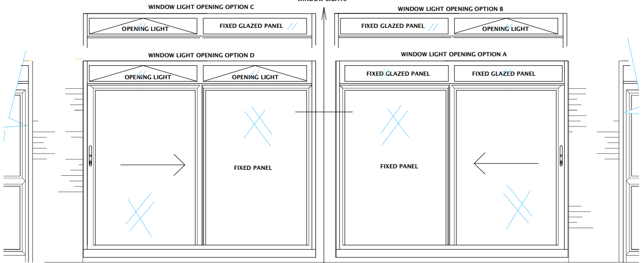
TWO STOREY HOUSE RIGHT SIDE OF BACK DOOR (FACING)
